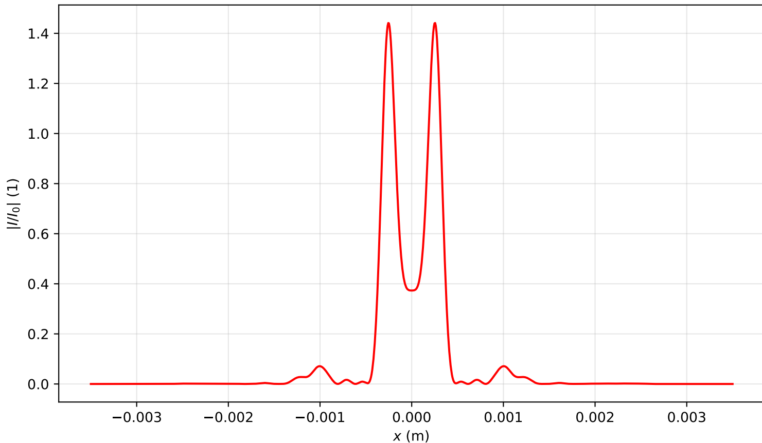
Intensity profile I(x, y = 0, z = 1.433)/I_0 , P_{in}=4.5P_{cr} , artificial time
